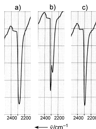
Figure 1. Part of the IR spectra of polymer-bound diazonium ions; the ν(N≡N) bands of the uncomplexed diazonium ion (a), as well as that of partly [18]crown-6 complexed (b), and that in the [21]crown-7 complex (c) are displayed.
