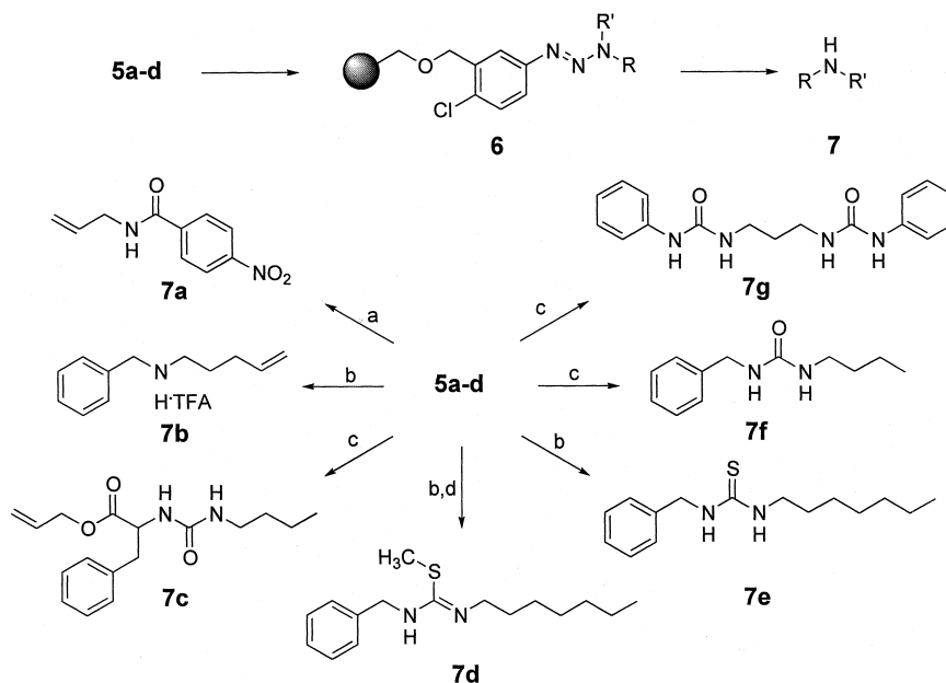
Scheme 3. The T2* resin as a linker in the synthesis of amine derivatives. a) Carboxylic acid chloride (1.5–2 equiv), pyridine, DMF, room temperature, 2 h; b) sodium hydride, DMF, electrophile (2–5 equiv), room temperature, 2 h; c) isocyanate (1.5–2 equiv), DMF, room temperature, 2 h; d) MeI, THF, room temperature, 30 min. Cleavage was conducted with 5% TFA in dichloromethane, room temperature, 5 min. The overall yield for attachment, modification, and cleavage of the amines was between 20 and 100%, generally greater than 80%, where the yields refer to the theoretically possible loading of the resin given by the starting material. Attachment of the linker and diazotization are considered as quantitative reactions, which was also confirmed by elemental analysis. After cleavage all products were obtained in > 95% purity, as determined by integration of the 1 H NMR signals and by HPLC analysis.
